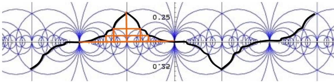
Fig. 2. Bidimensional pattern of a j-function, displaying the real part of j-oscillations. The black line depicts the j-pattern correlated with EEGs traces.
