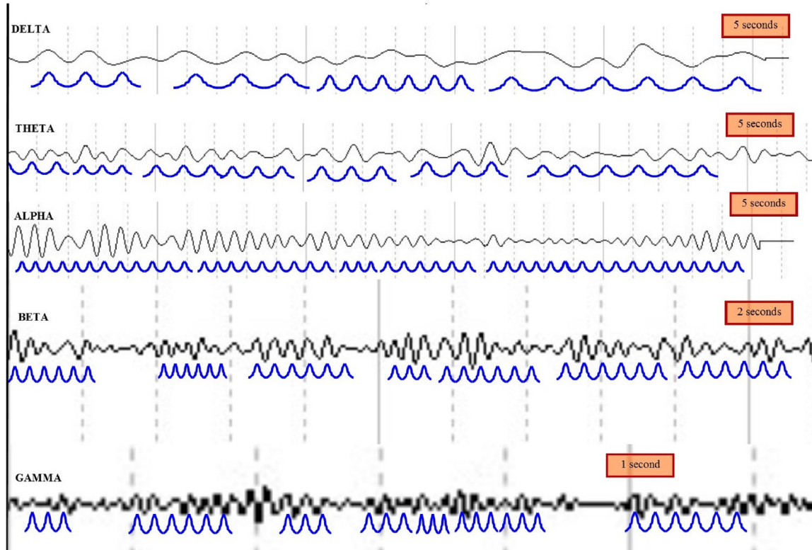
Fig. 3. Relationships between the j-function pattern (blue waves) and normal EEG rhythms (black waves) in the FZ- derivation of a single male control. The predicted blue curves match with the normal EEG oscillations almost everywhere. Delta, theta and alpha traces have the same resolution for the y (microV) axis, which gives a rather unclear view for the beta and gamma waves, usually in the <1 mV range. Therefore, beta and gamma frequencies are depicted in Figure at higher magnification and with a different temporal scale. (For interpretation of the references to colour in this figure legend, the reader is referred to the web version of this article.)
